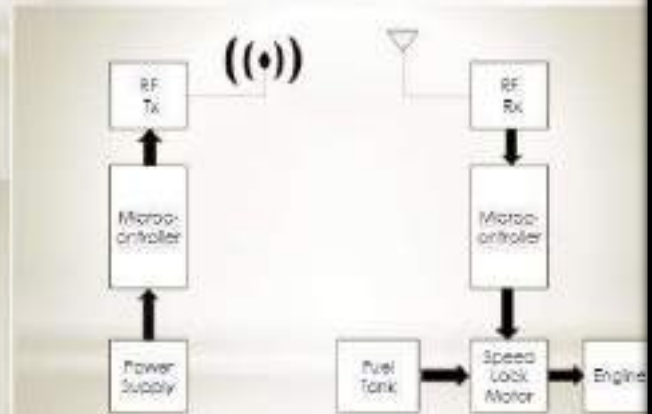
Figure 4 : Block diagram
